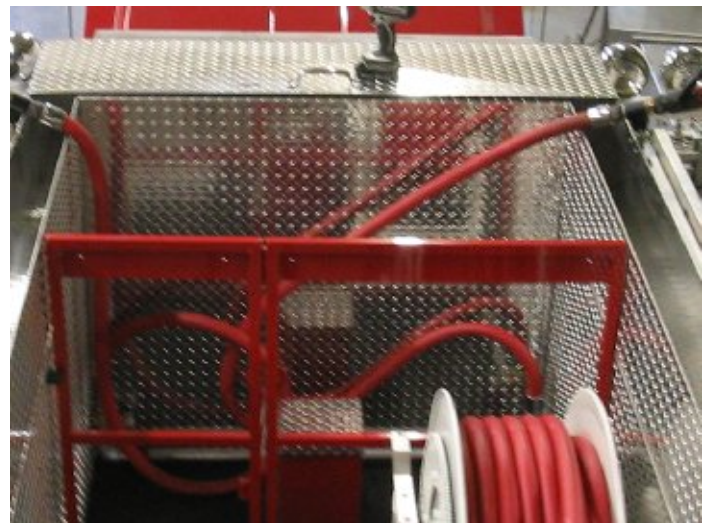
RIDER TURRET CAGE & STORAGE CABINET IN HEATSHIELD
