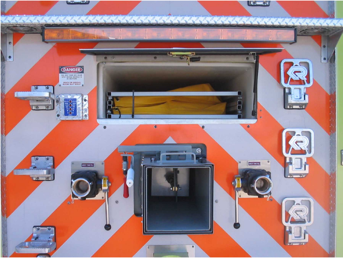
2-2 1/2" QUICK FILLS, 10 X 10 QUICK DUMP, FOLDING TANK STORAGE & REAR WATER LEVEL INDICATOR REAR TRAFFIC ADVISOR WITH FULL WIDTH REAR INTERMEDIATE HOSEBED ACCESS STEP MAIN HOSEBED HINGED ALUMINUM COVER & VINYL END FLAPS WITH HANDRAILS & FOLDING STEPS
